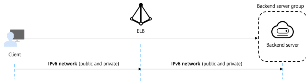
Figure 3-1 Network types supported by dedicated load balancers at Layer 4
